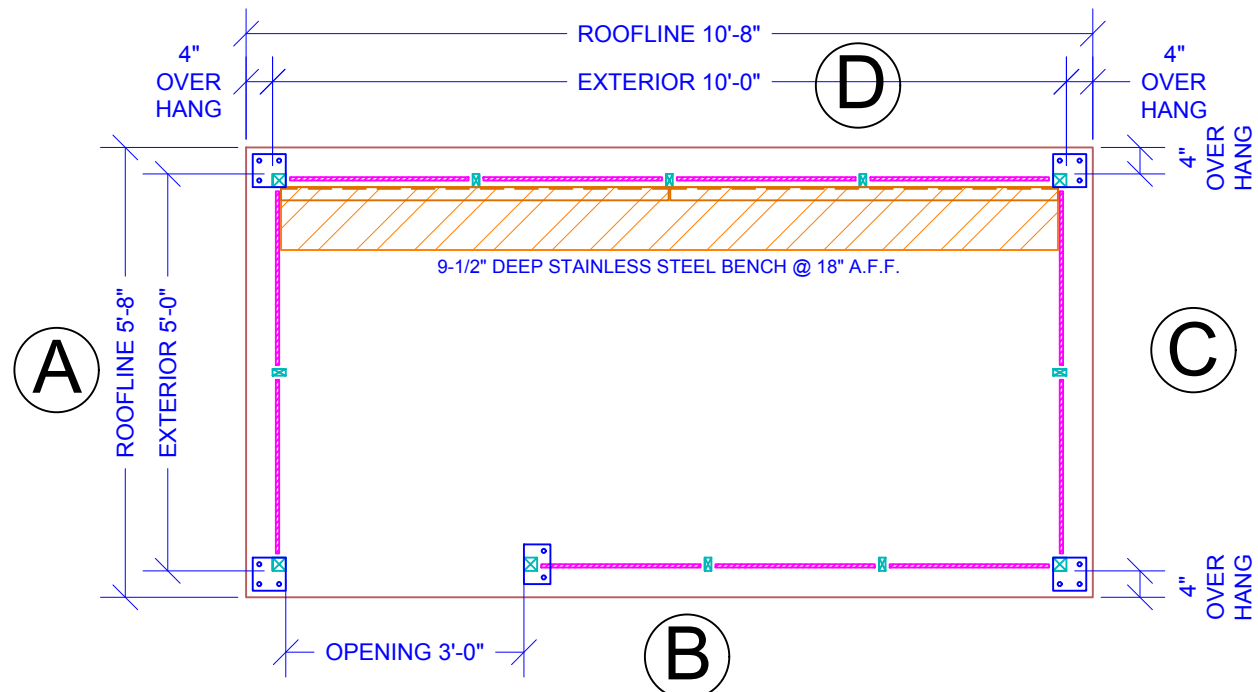
5'X10' STEEL SHELTER PLAN VIEW
