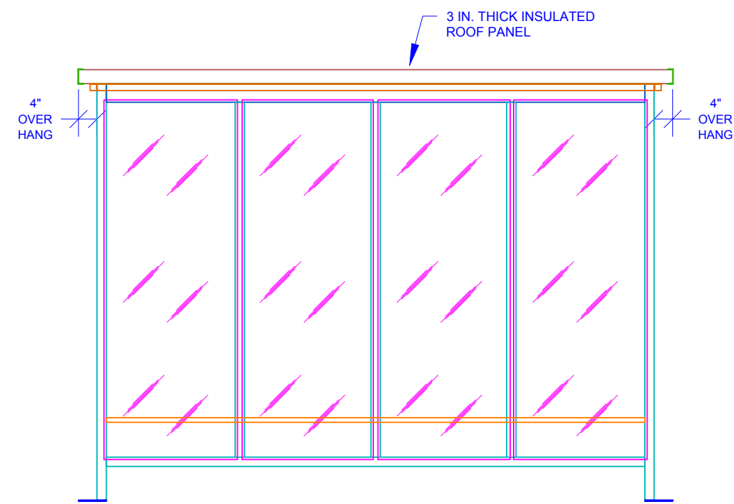
ELEVATION D
