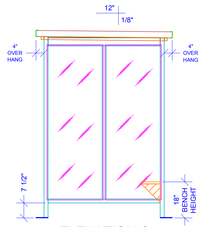
ELEVATION C
